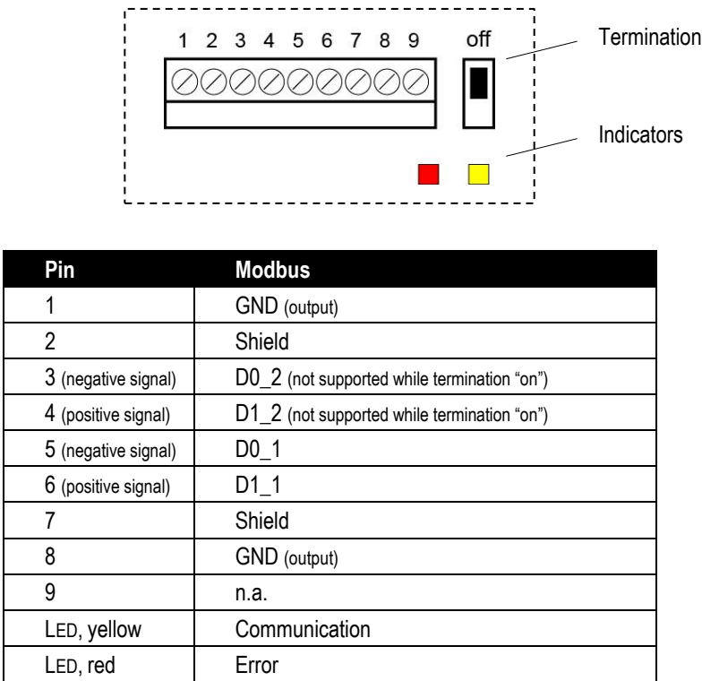
Figure 87: Terminal for Comm Box (DIN 6TE)
