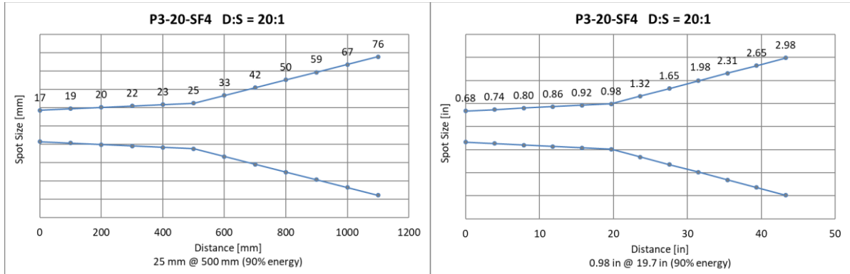
Figure 15-14: Optical Diagrams P3-20 Models
