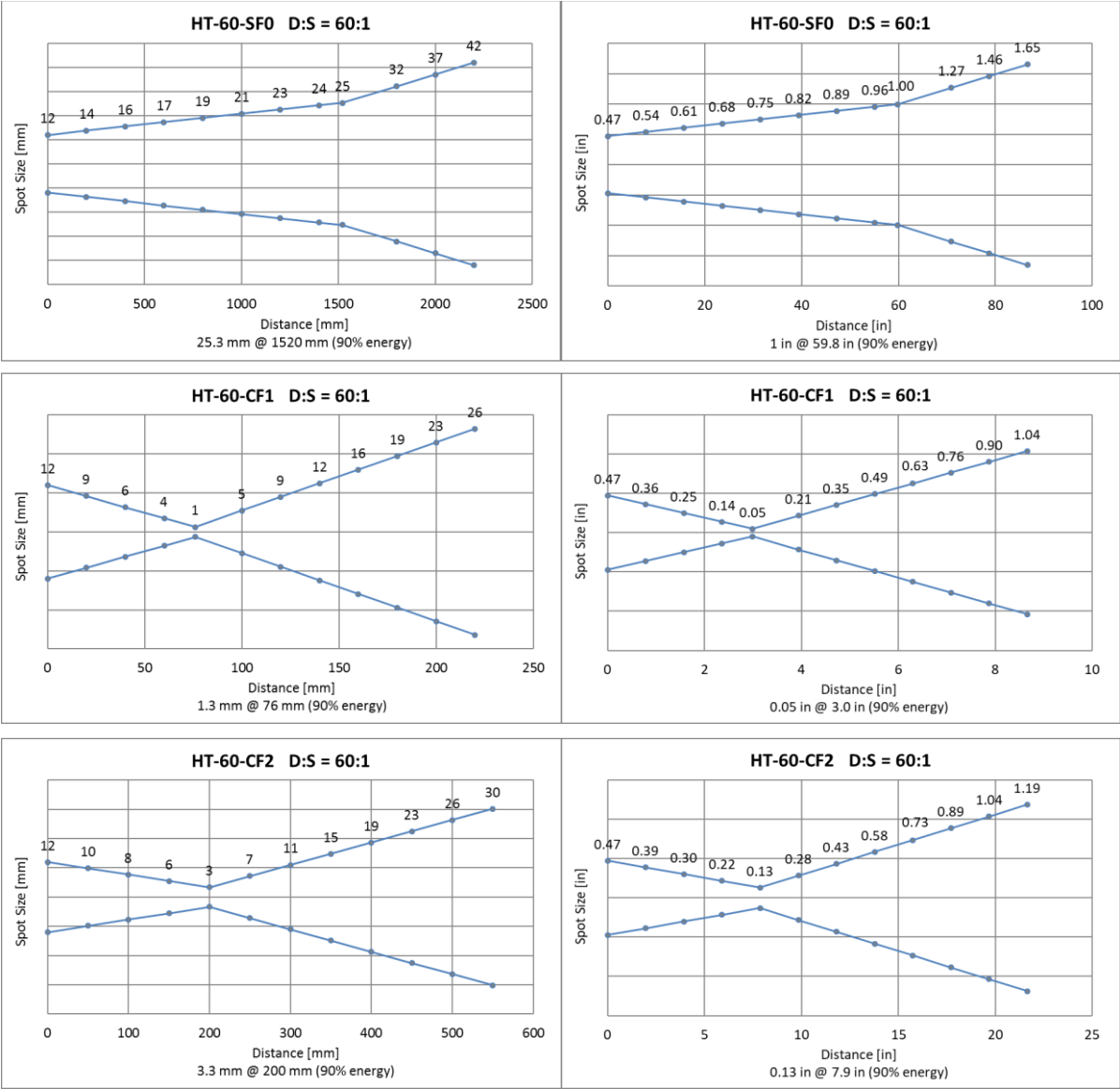
Figure 15-15: Optical Diagrams HT-60 Models
