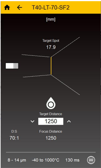
Figure 15-19: Spot Size Calculator
