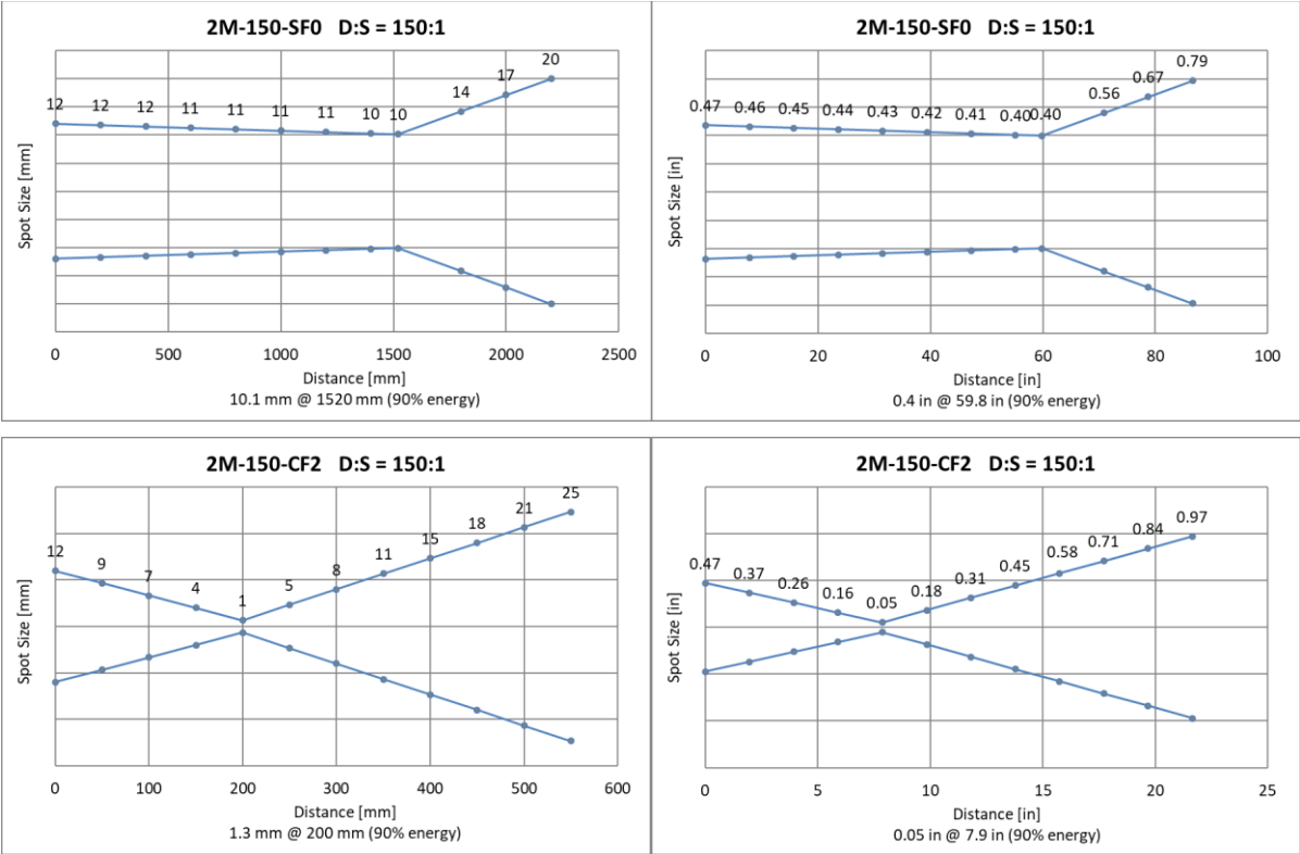
Figure 15-17: Optical Diagrams 2M-150 Models
