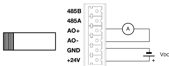
Figure 5-13: Wiring Analog Out as Current Output
