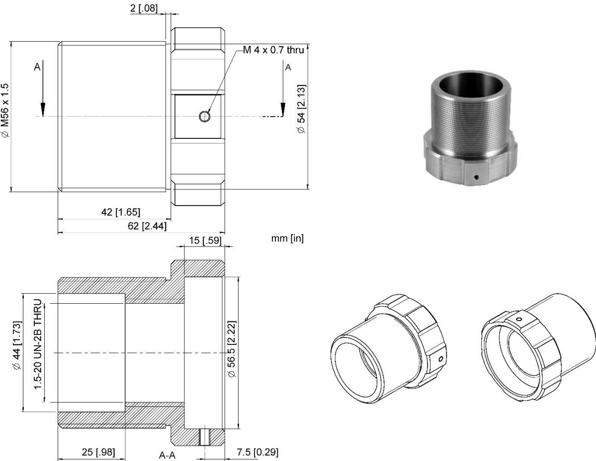
Figure 13-24: Thread Adapter
