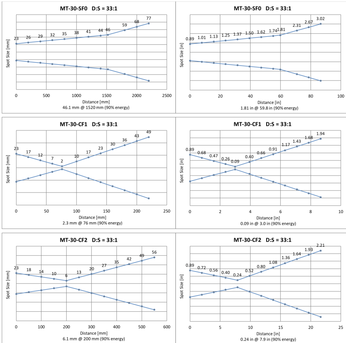
Figure 15-12: Optical Diagrams MT-30 Models
