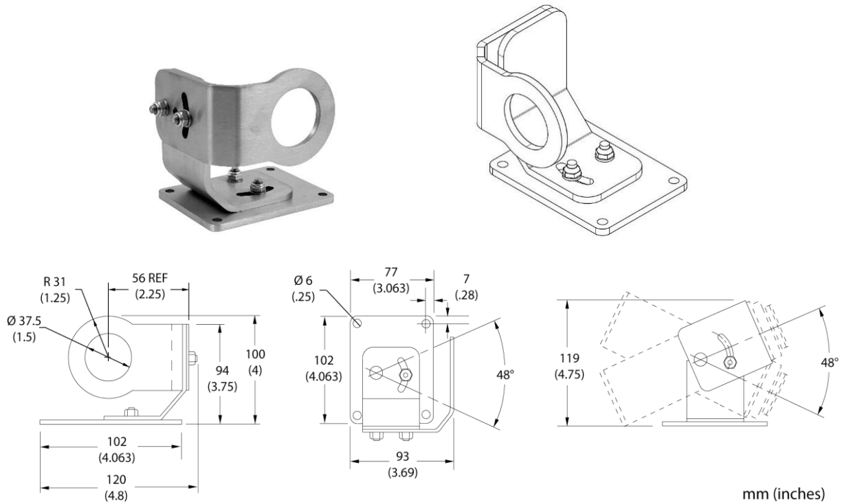
Figure 13-14: Adjustable Bracket
