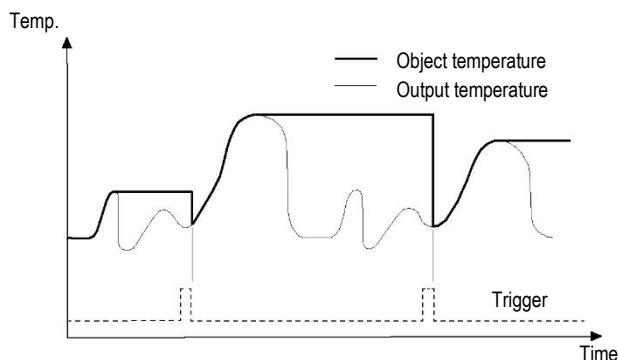
Figure 5-21: Holding the Output Temperature
