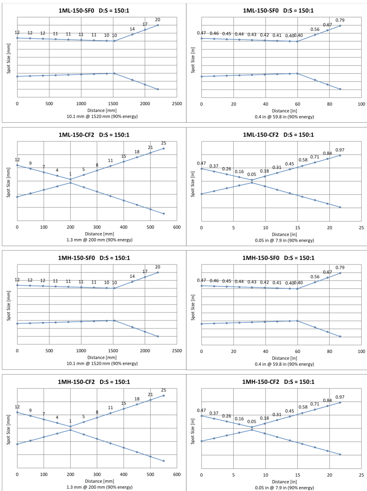
Figure 15-16: Optical Diagrams 1M-150 Models
