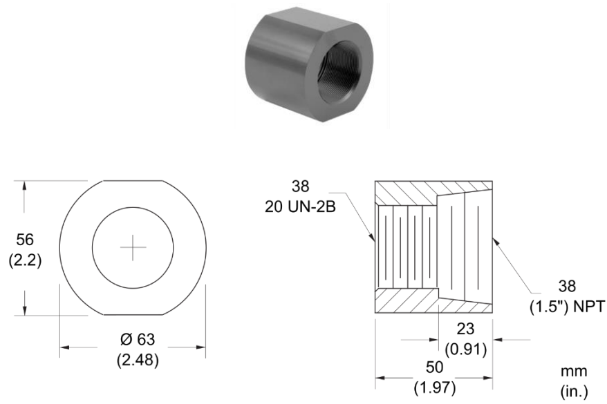
Figure 13-19: Pipe Adapter
