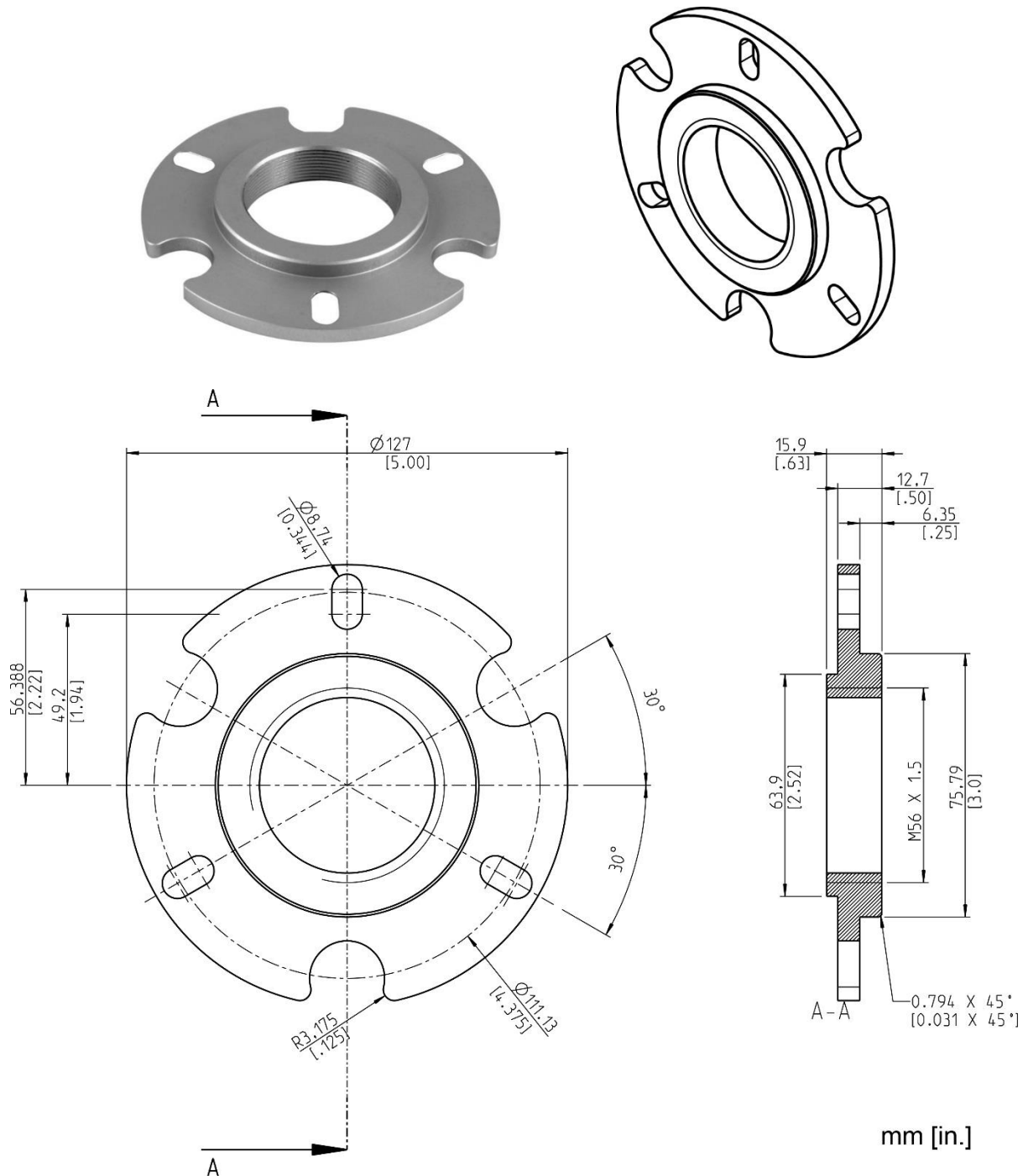
Figure 13-25: Mounting Flange
