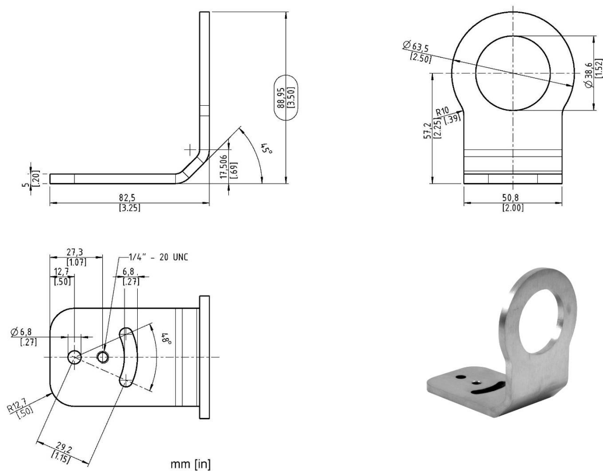
Figure 13-13: Fixed Bracket
