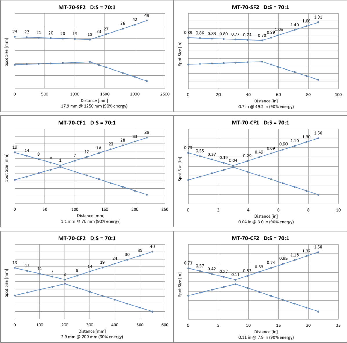
Figure 15-13: Optical Diagrams MT-70 Models
