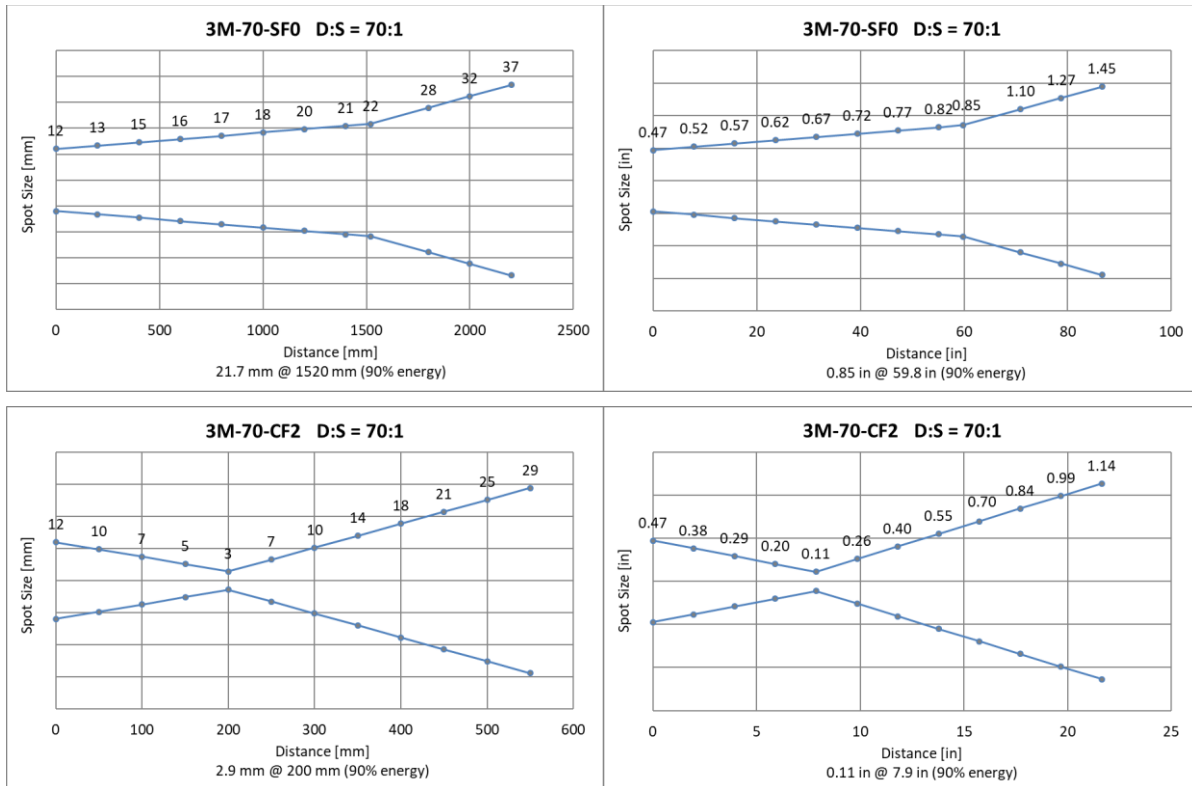
Figure 15-18: Optical Diagrams 3M-150 Models
