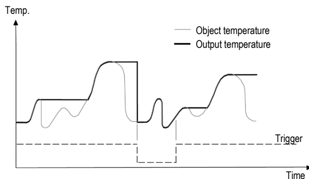
Figure 5-20: Resetting the Peak Hold Function
