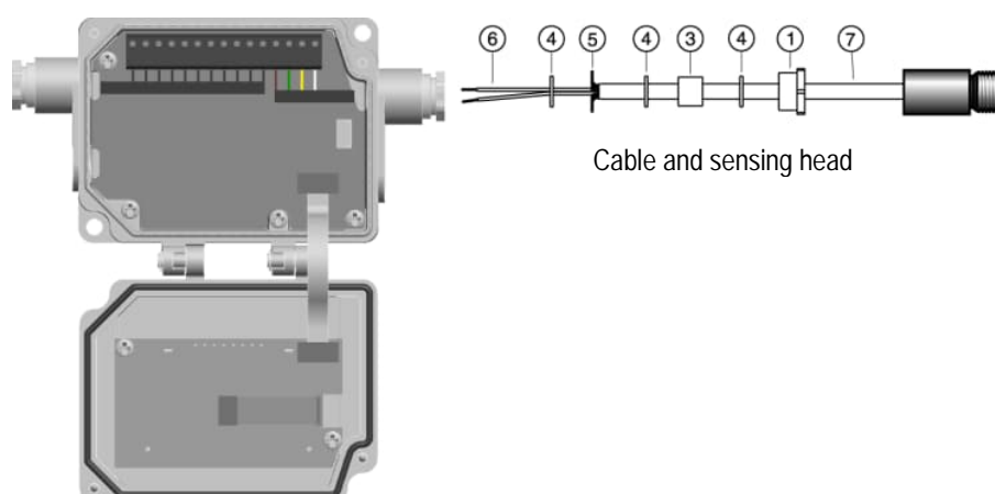
Figure 13: Sensing Head Cable to the Comm Box
